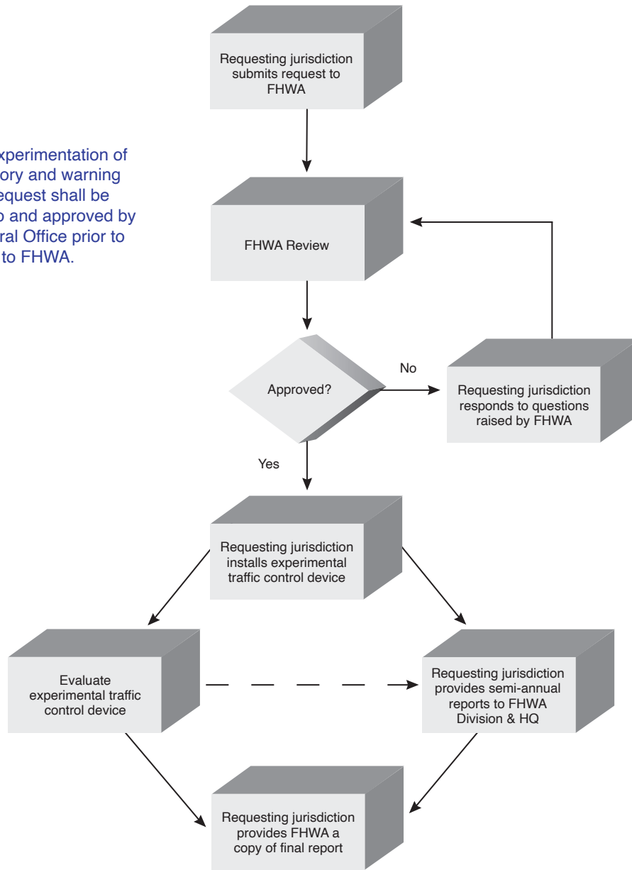
Figure 1B-1(VA). Process for Requesting and Conducting Experimentations for New Traffic Control Devices
